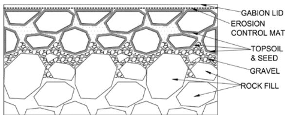
GABION SECTION
