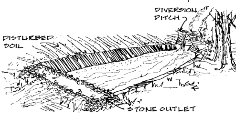
(Graphic from MA Unpaved Road BMP Guide)
