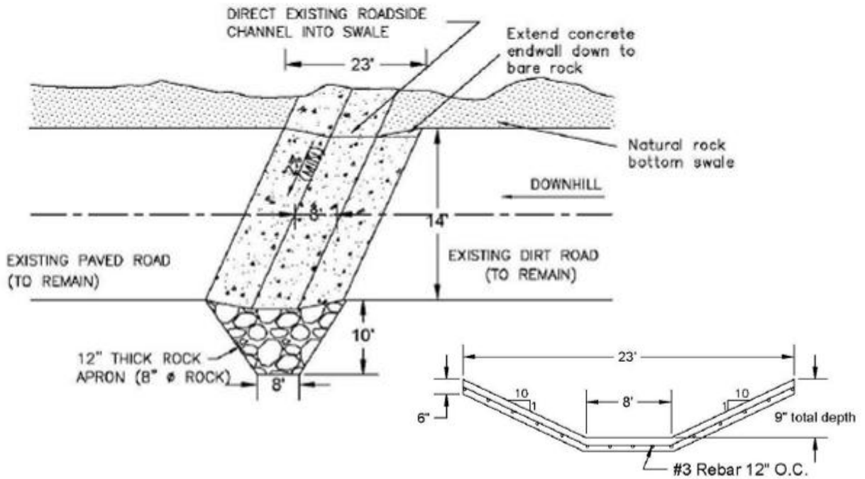
(Source: Coral Bay Community Council)
