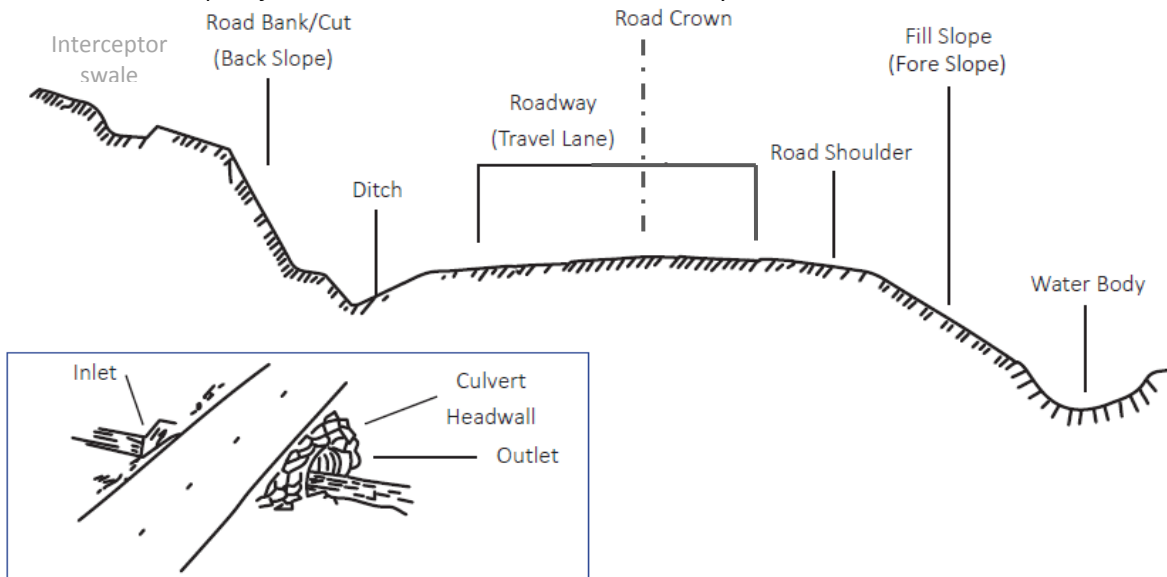
Figure 1. Features of a Road
