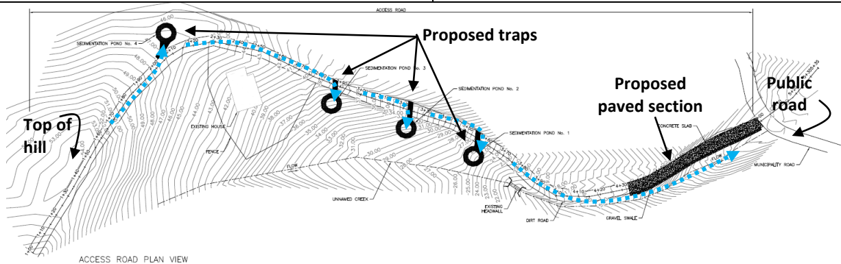
Turnouts & waterbars used to divert flows into four sediment traps along a steep unpaved access road on Culebra.
