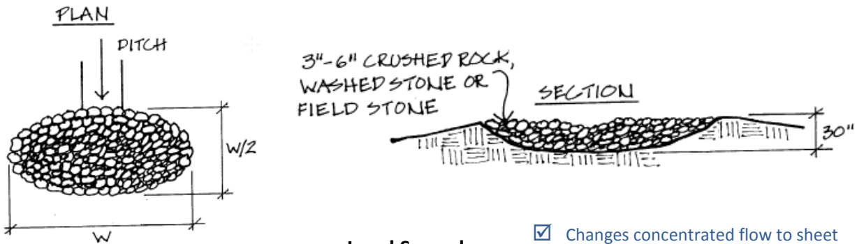
Level Spreader
