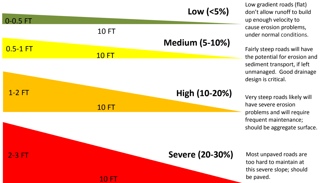
Figure 2. Road Steepness and Erosion Risk (adapted from the Vermont Better Backroads Manual, 2009)
