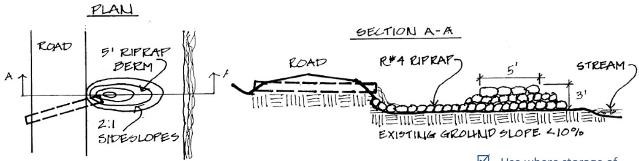
Plunge Pool
