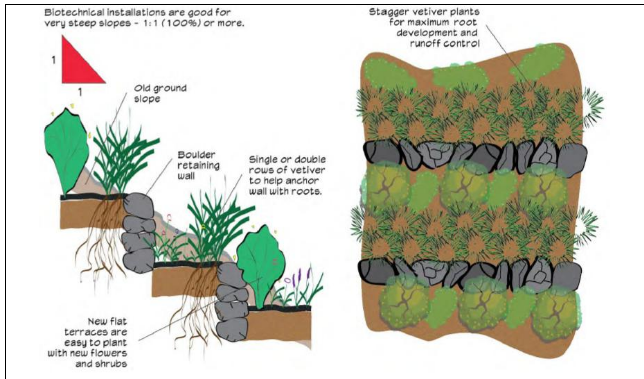
Combination of terracing, retaining walls, and vetiver to stabilize a slope (Coral Bay Community Council, 2017).
