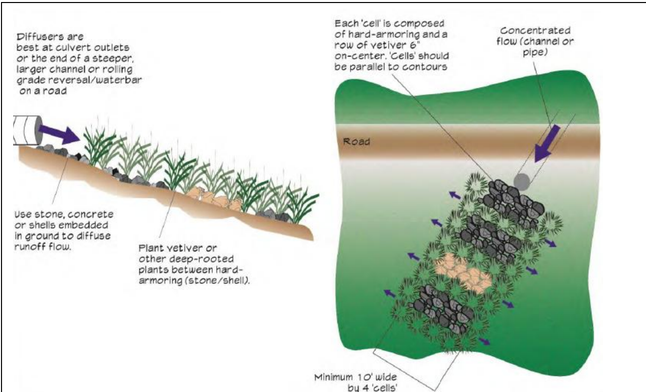
Vetiver diffuser detail from Coral Bay Community Council (2017) used to dissipate energy and disperse concentrated flows at the end of a pipe, waterbar, dip, etc. Rows should be a minimum width of 10 feet.
