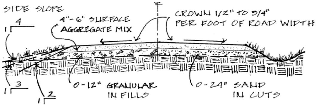
Figure 4. Unpaved Road Surfacing
