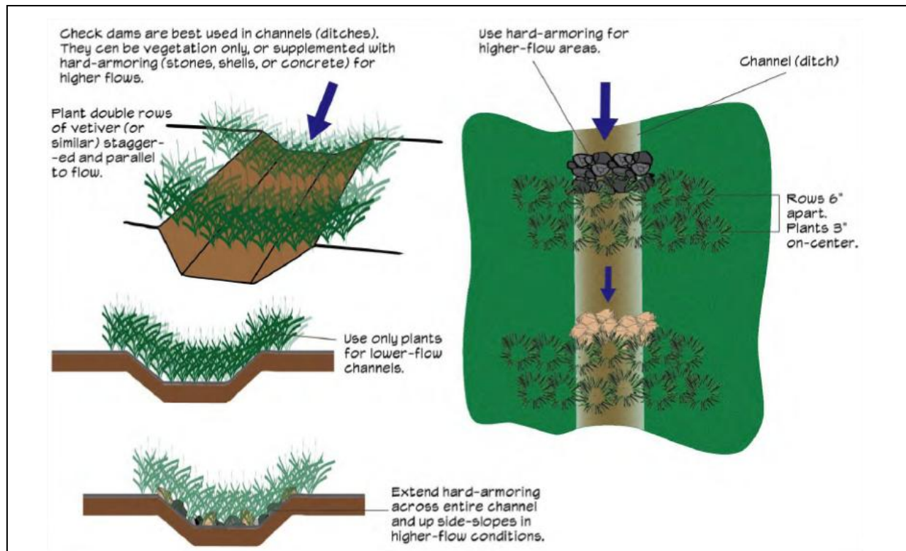
Vetiver check dam detail with armoring options for higher flow channels (from Coral Bay Community Council, 2017). The vetiver grass helps dissipate energy, trap sediment, and soak up standing water.
