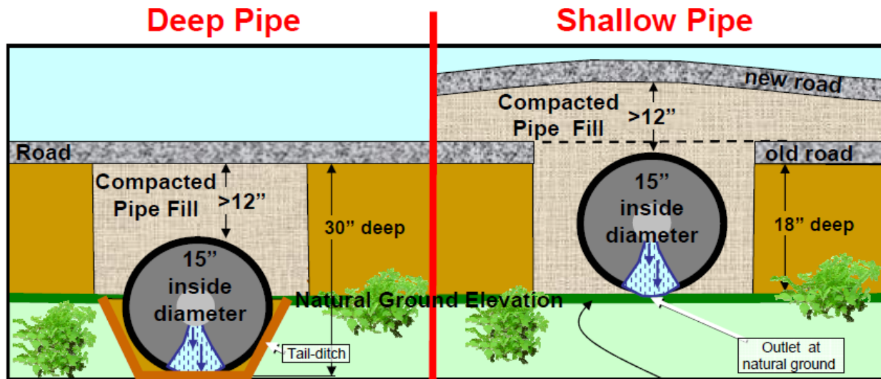
Side View, looking through crosspipe from outlet, comparing deep and shallow pipe placements. Note the green "natural ground elevation" line. Deep pipes dig down to obtain pipe cover. Shallow pipe placements are based off the natural ground elevation, and use fill to achieve pipe cover.
