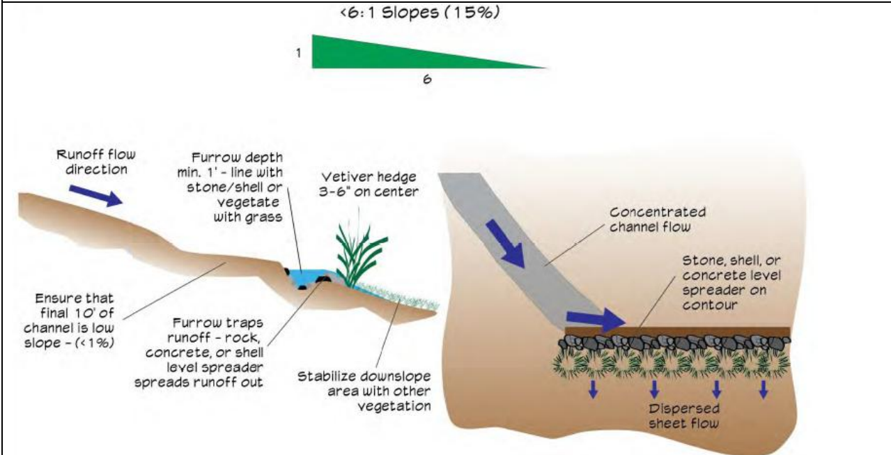
Vetiver spreader system detail from Coral Bay Community Council (2017) showing option for converting concentrated flow to sheet flow using rock, shell, or concrete level spreader. Good for turnouts and other flows on slopes of 15% or less.
